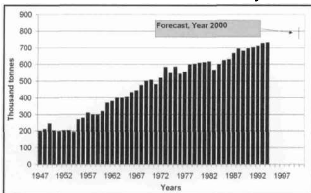
Figure 1. World elasmobranch catches according to FAO statistics with forecasted catches for year 2000.
