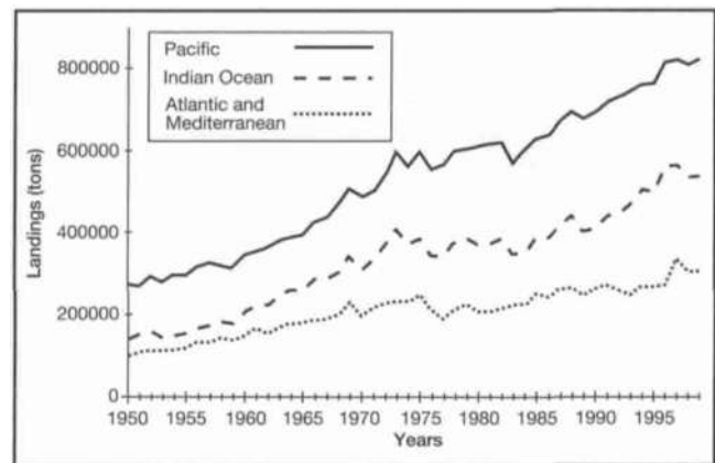
Figure 4. FAO nominal catches for elasmobranchs by selected FAO statistical areas. A continuous decline in catches in the Northwest Pacific is compensated by increased catches in the Western Central Pacific.
