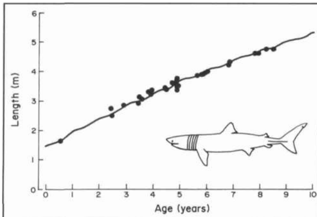
Figure 4. Seasonally oscillating growth curve of basking sharks in the North Atlantic, based on lengths plotted sequentially against the corresponding months of capture or stranding. Based on data in Table 2. Note that plotting the second smallest point one year earlier would lead to an extremely 'fast' growth curve, not supported by the rest of the sequence, and inconsistent with alternating periods of fast summer growth and reduced winter growth.
