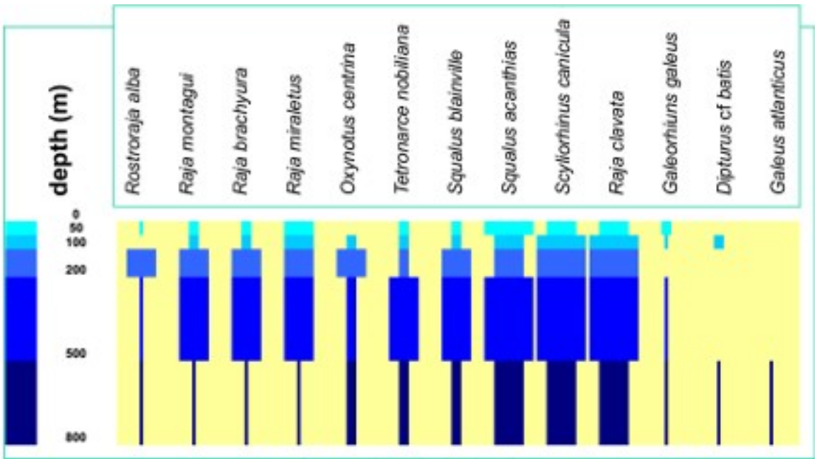
Fig. 4. Species on the whole depth range. Bar width represents the density index with the ranges: <0.1, 0.1-1, 1-10, >10 kg/km².
