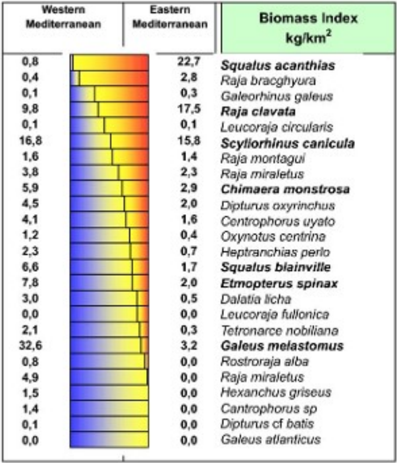
Figure 5. Distribution of biomass indexes (kg/km²) in the European Mediterranean related to their east-west gradient.
